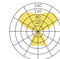
flat (2x55W) η = 79,1% cd/1000lm
