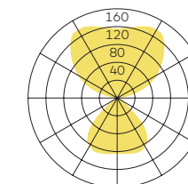
flat (2x54W) η = 81,5% cd/1000lm
