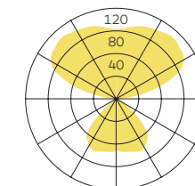
flat (2x54 W), (2x80W) η = 75,3% cd/1000lm
