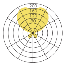
twilight (8027) 94lm/W@2700K
